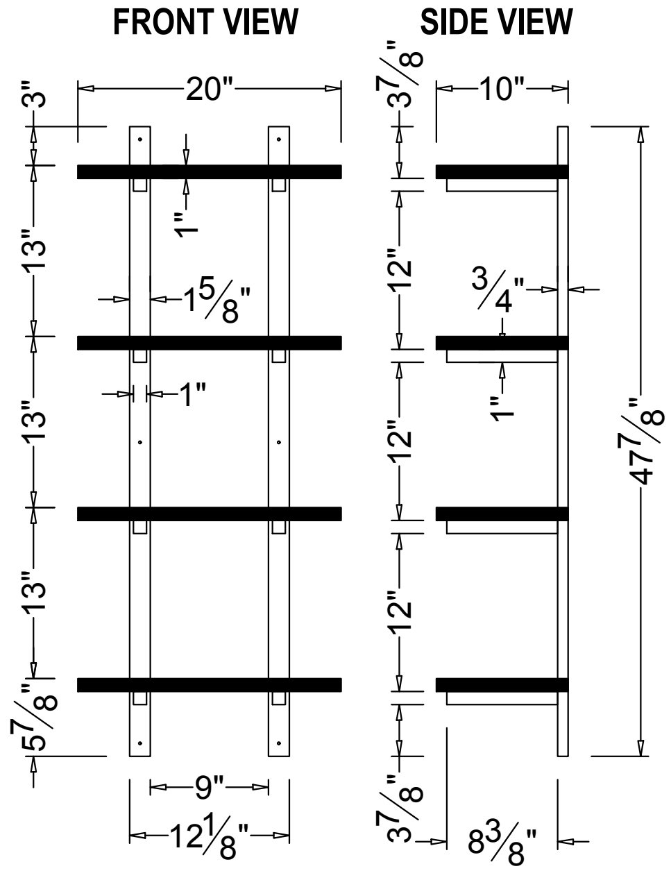
AMBA5620 POMONA LIVING ROOM 20*48 WALL STORAGE
